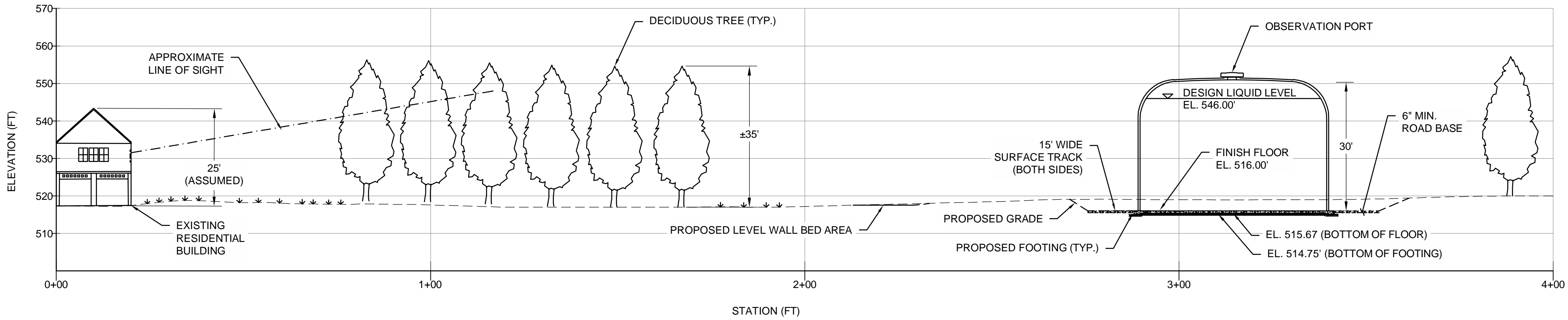
SECTION B-B'
