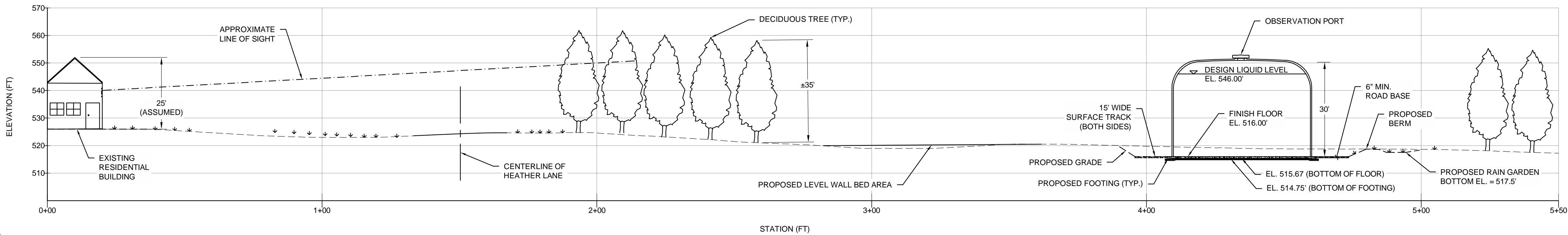
SECTION C-C'
